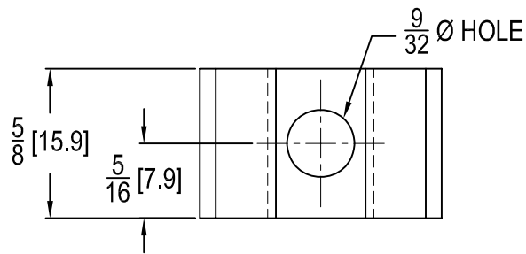
AW0923 Mat'l. : BRASS
